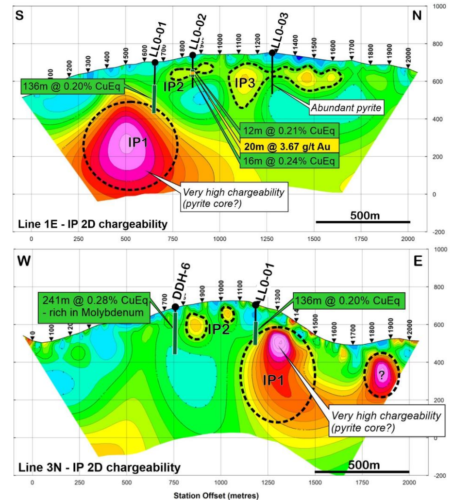
Main IP Chargeability-MT Resistivity anomalies
