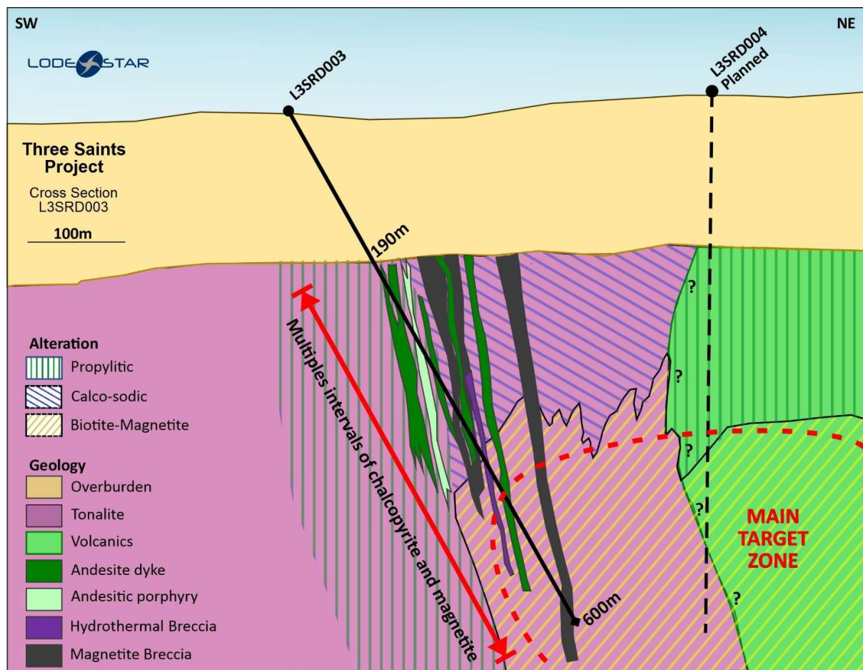
Figure 5: Cross Section of L3SRD003, showing the logged geology and alteration.
